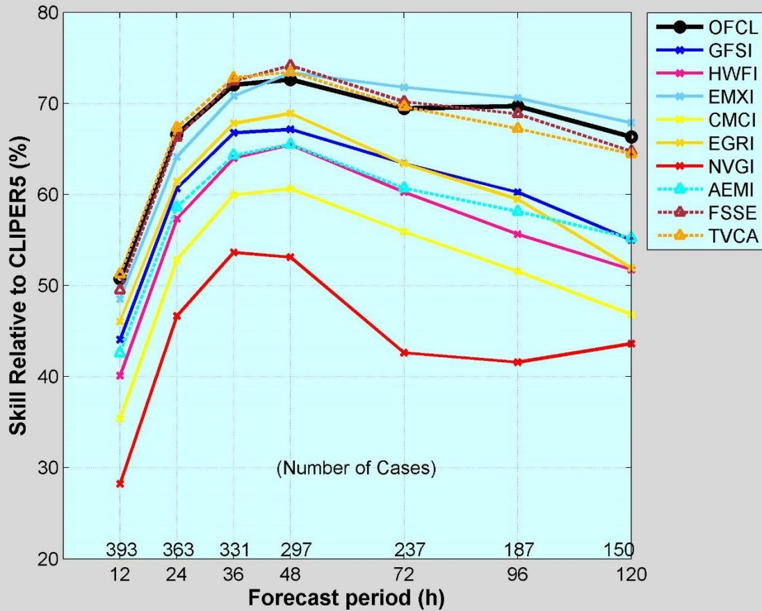
Track Forecast Skill (Early Models) 2015-17 - Atlantic Basin
