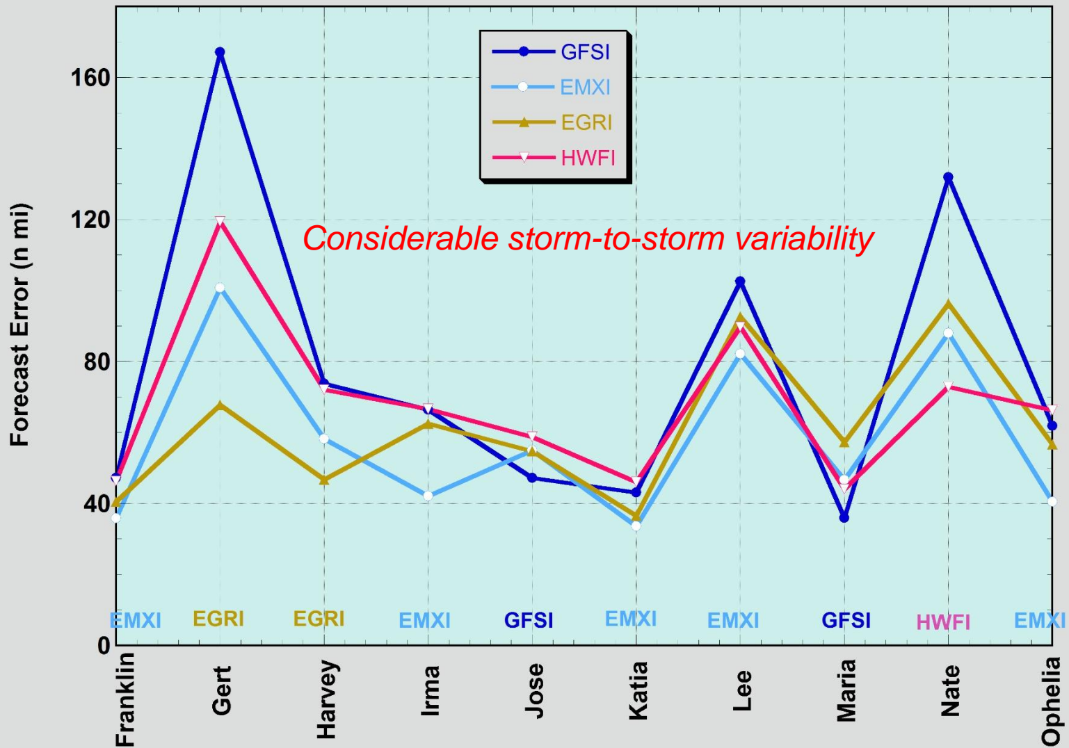
48-h Track Model Forecast Errors by Storm 2017 - Atlantic Basin
